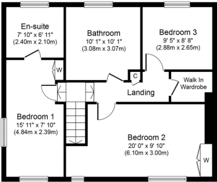
First Floor Approximate Floor Area 646 sq. ft. (60.0 sq. m.)
